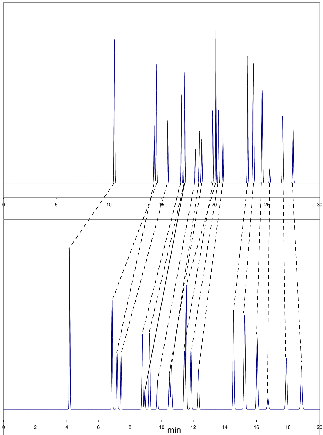
Figure 3: Changes in the elution pattern due to changes in the initial condition of gradients with the same gradient slope. (© Uwe Neue, Waters Corp)
