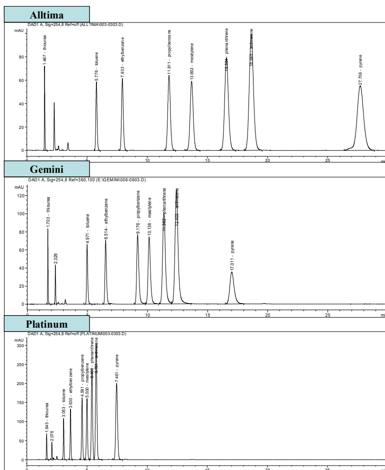
Fig.1. Separation of a neutral test mixture of alkylbenzenes and polynuclear aromatic hydrocarbons on three nominal identical C-18 RPLC columns. Test conditions as for test 1; test analytes are indicated in the figure; thiourea is used as dead time marker.
