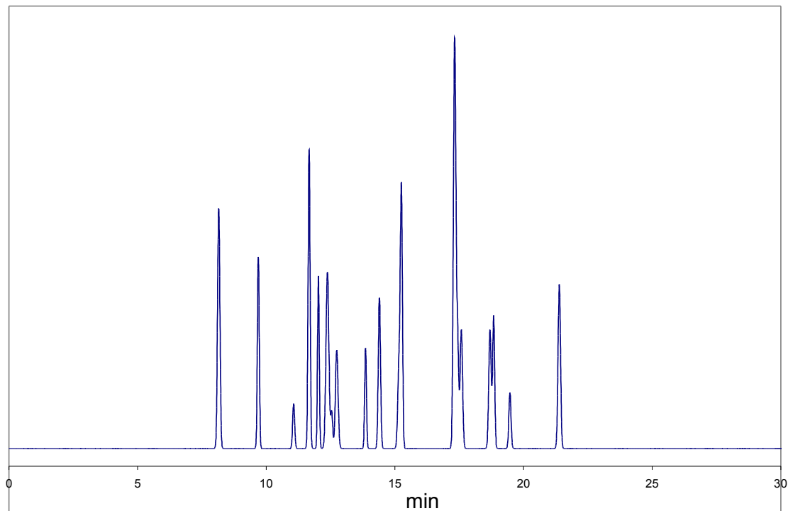
Figure 6: Simulated chromatograms with (top) and without (bottom) peak compression. (© Uwe Neue, Waters Corp)
